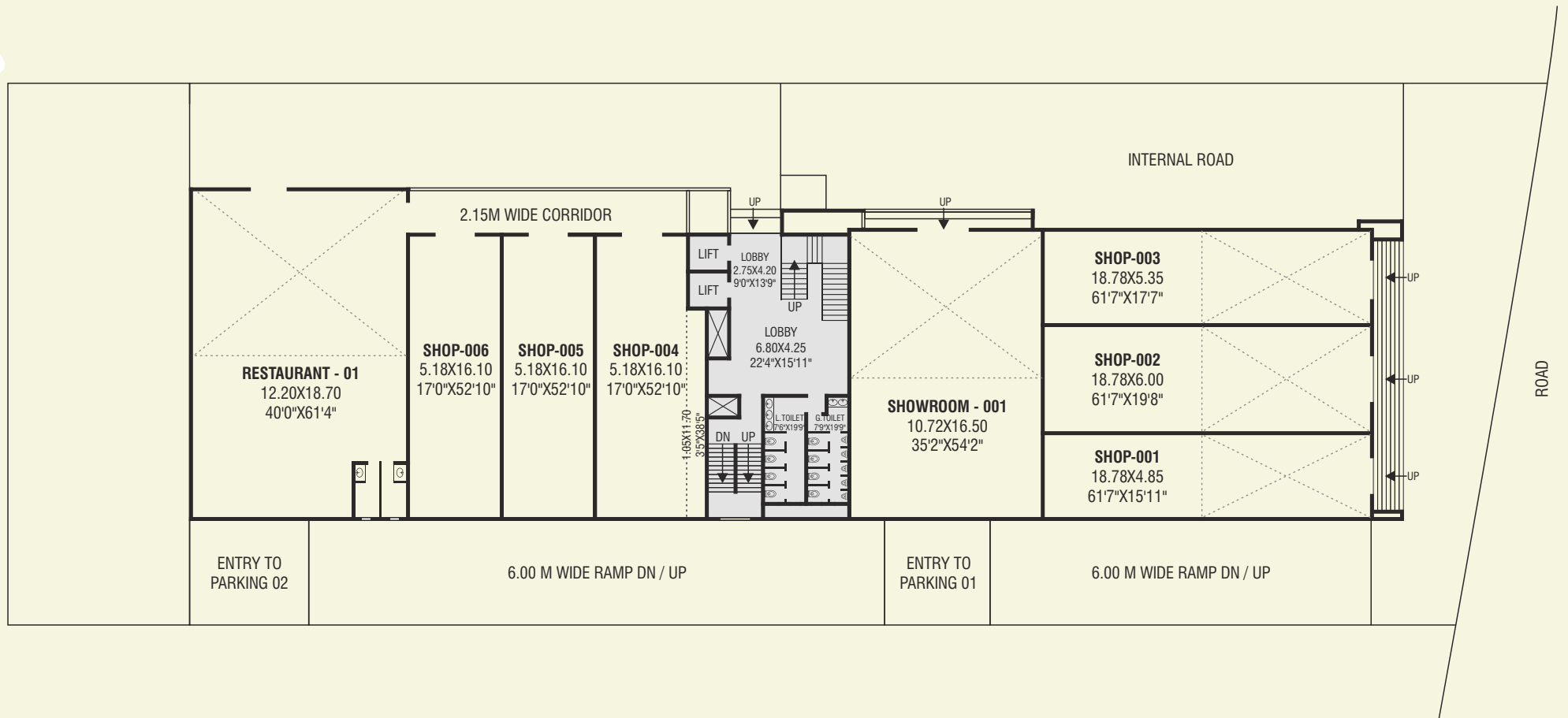
GROUND FLOOR : Area Statement
